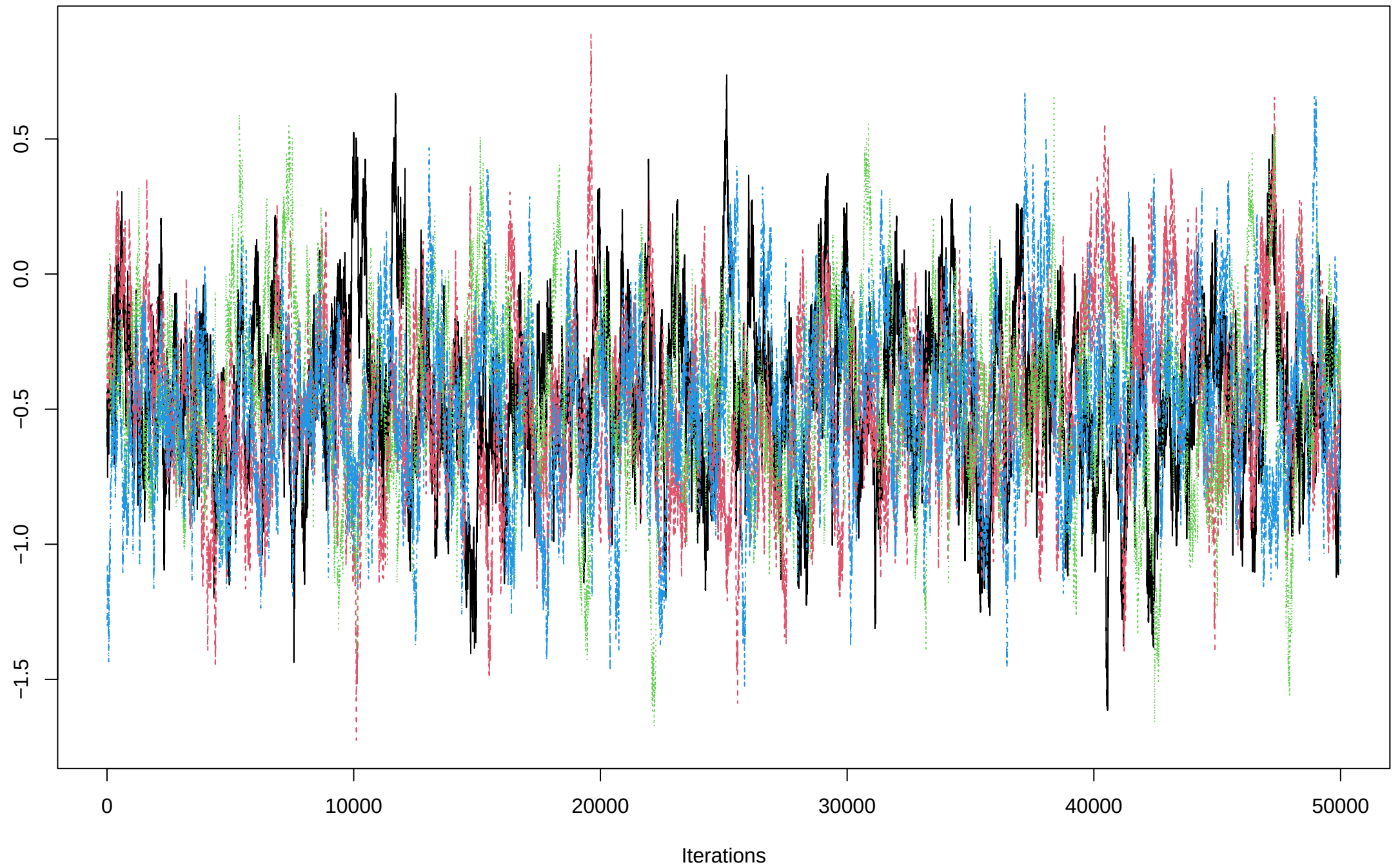
Trace of a[3]
