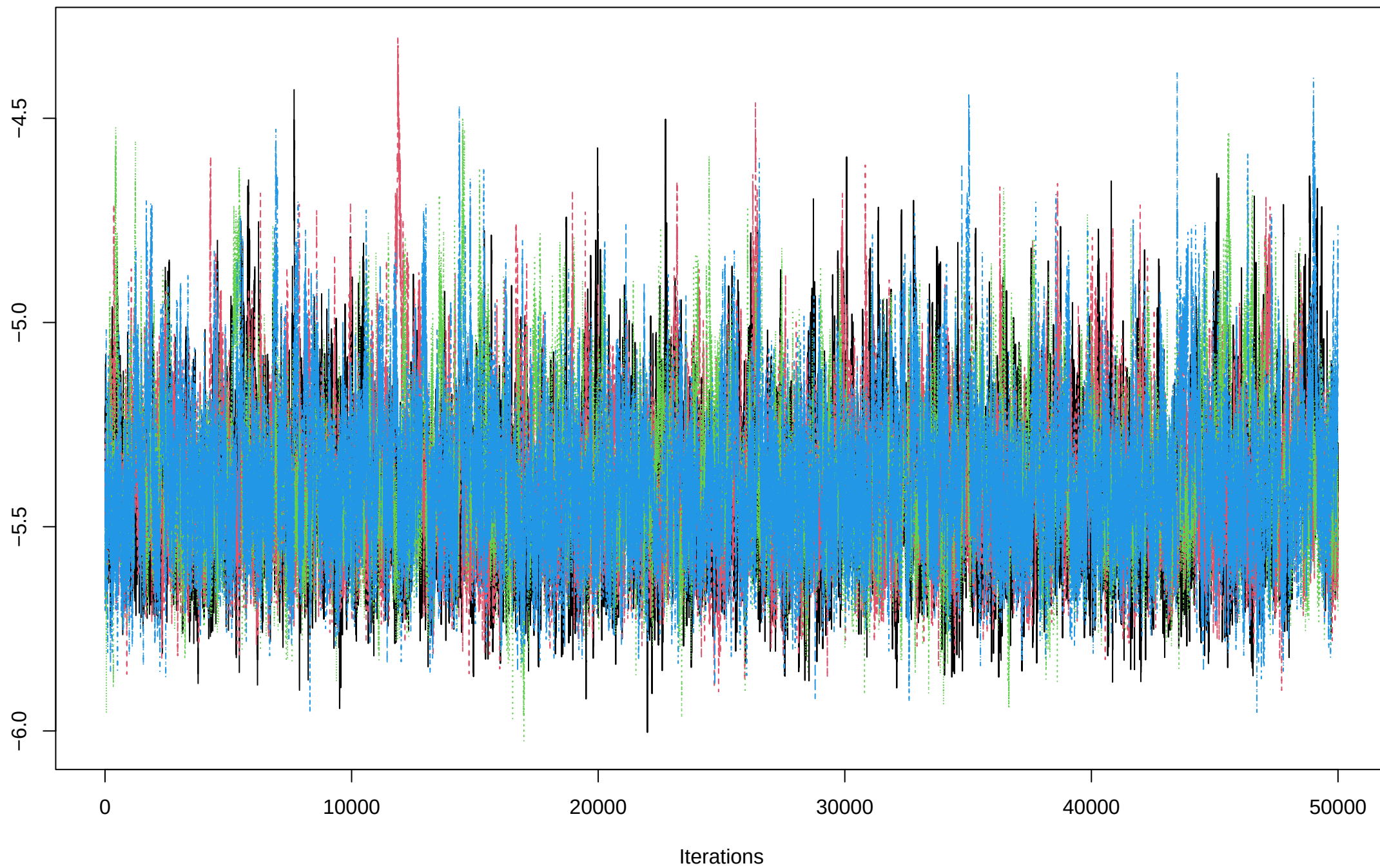
Trace of a[1]
