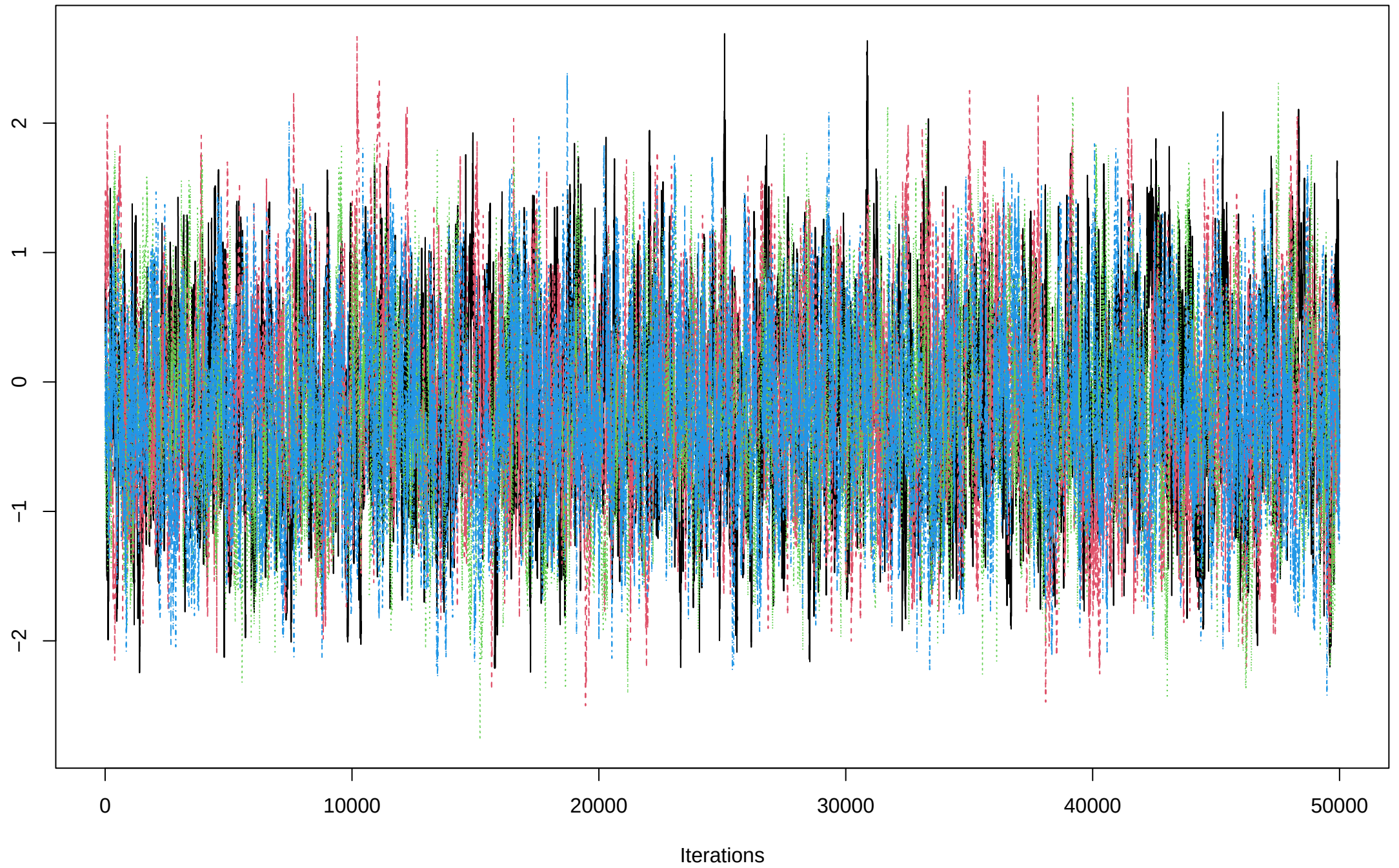
Trace of b[2]
