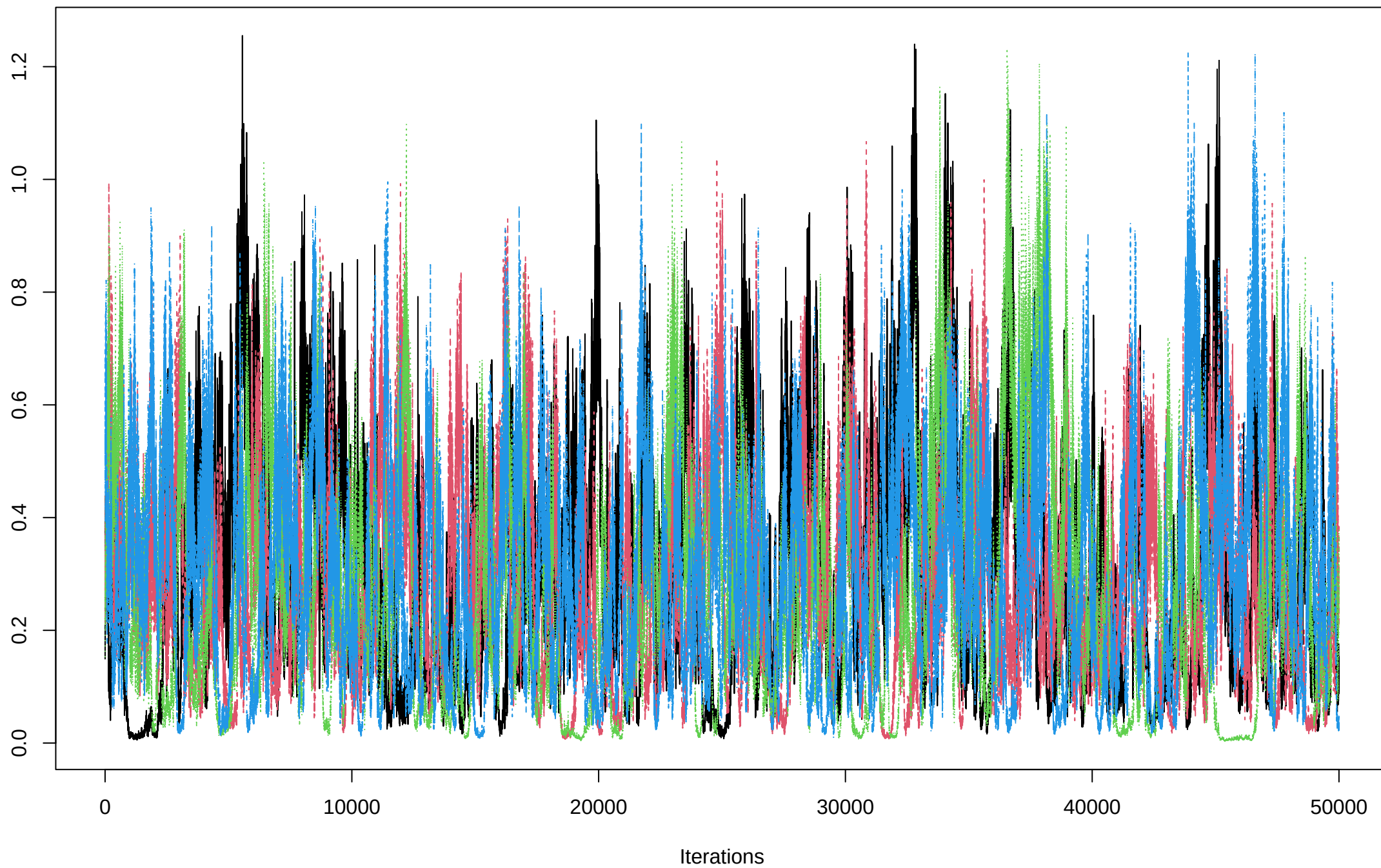
Trace of sigma
