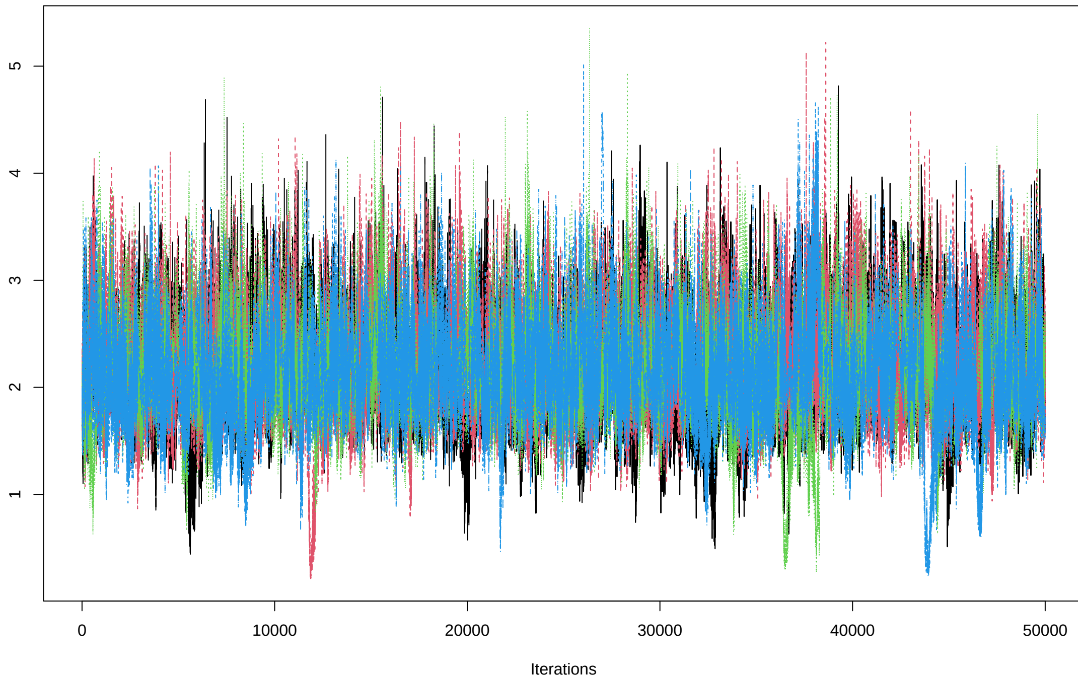
Trace of nu
