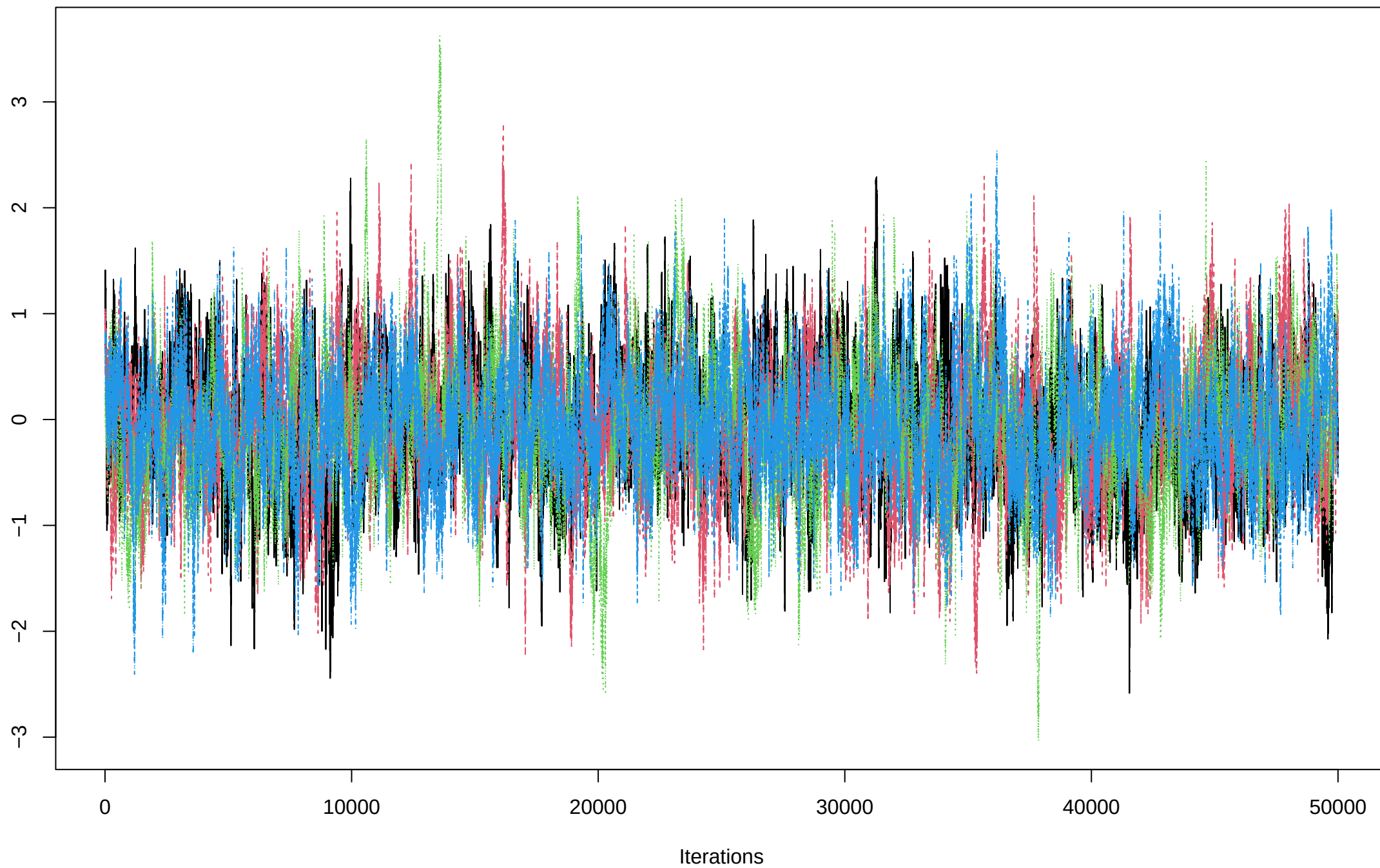
Trace of phi[17]
