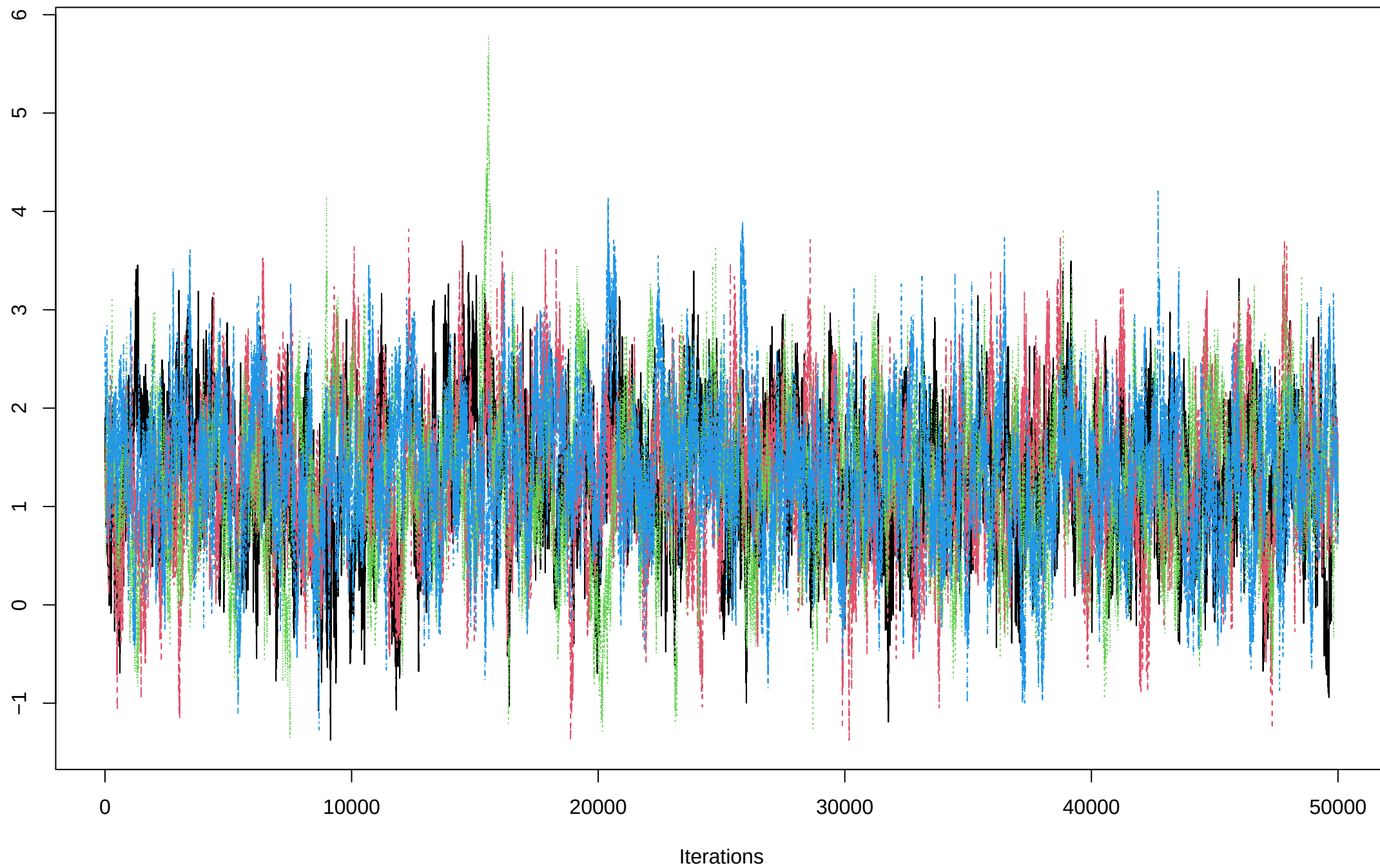
Trace of phi[1]
