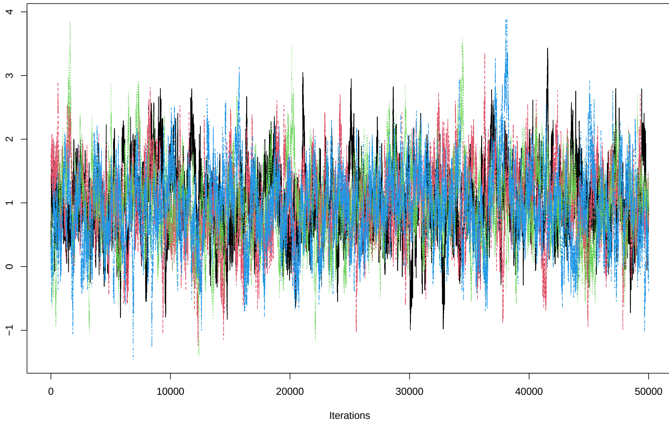
Trace of phi[10]
