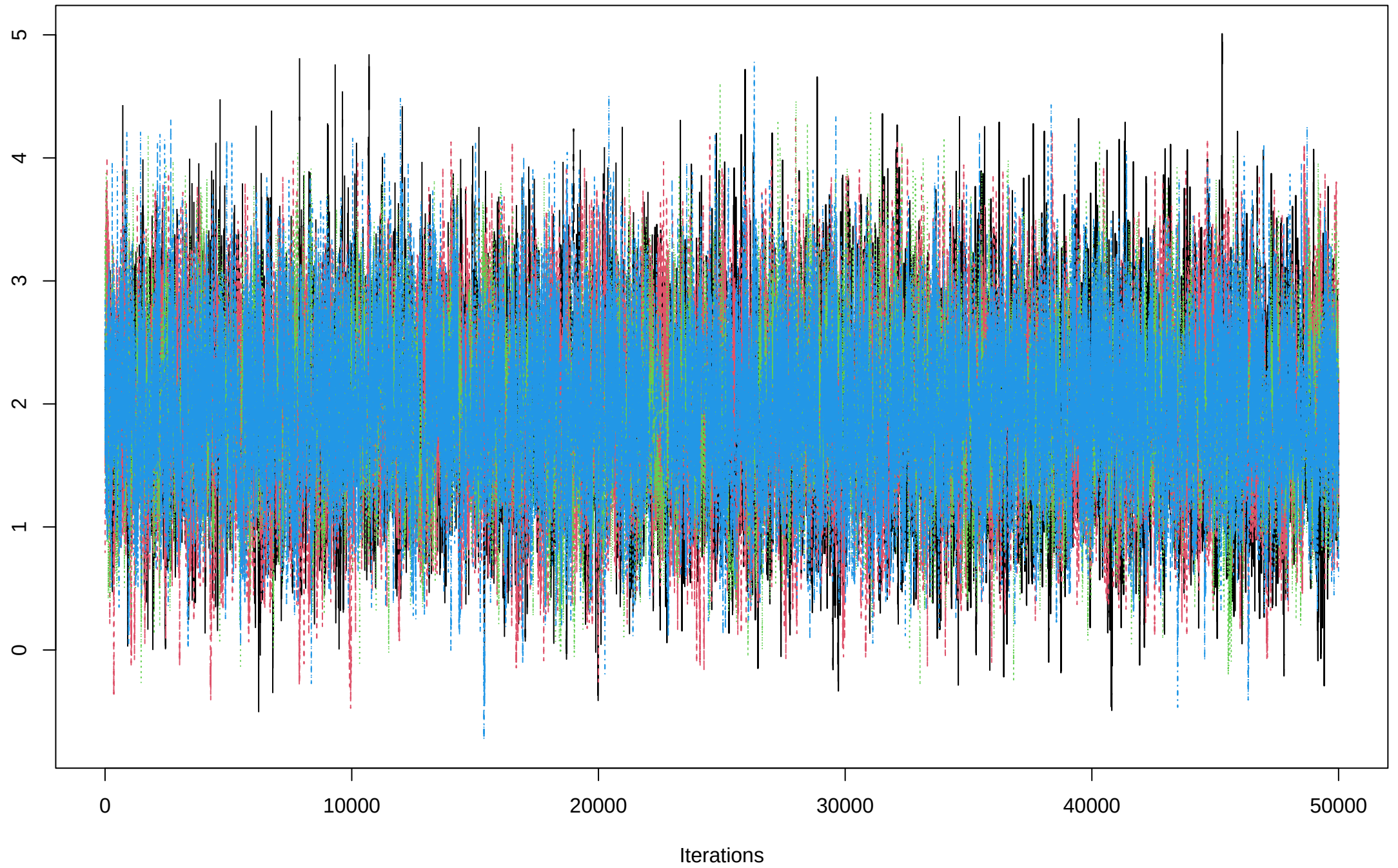
Trace of b[1]
