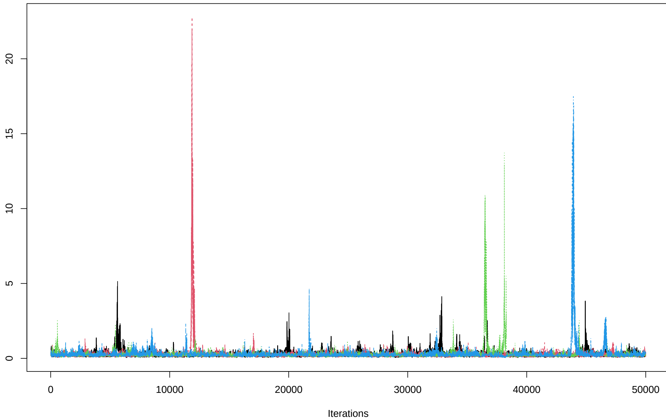
Trace of tau
