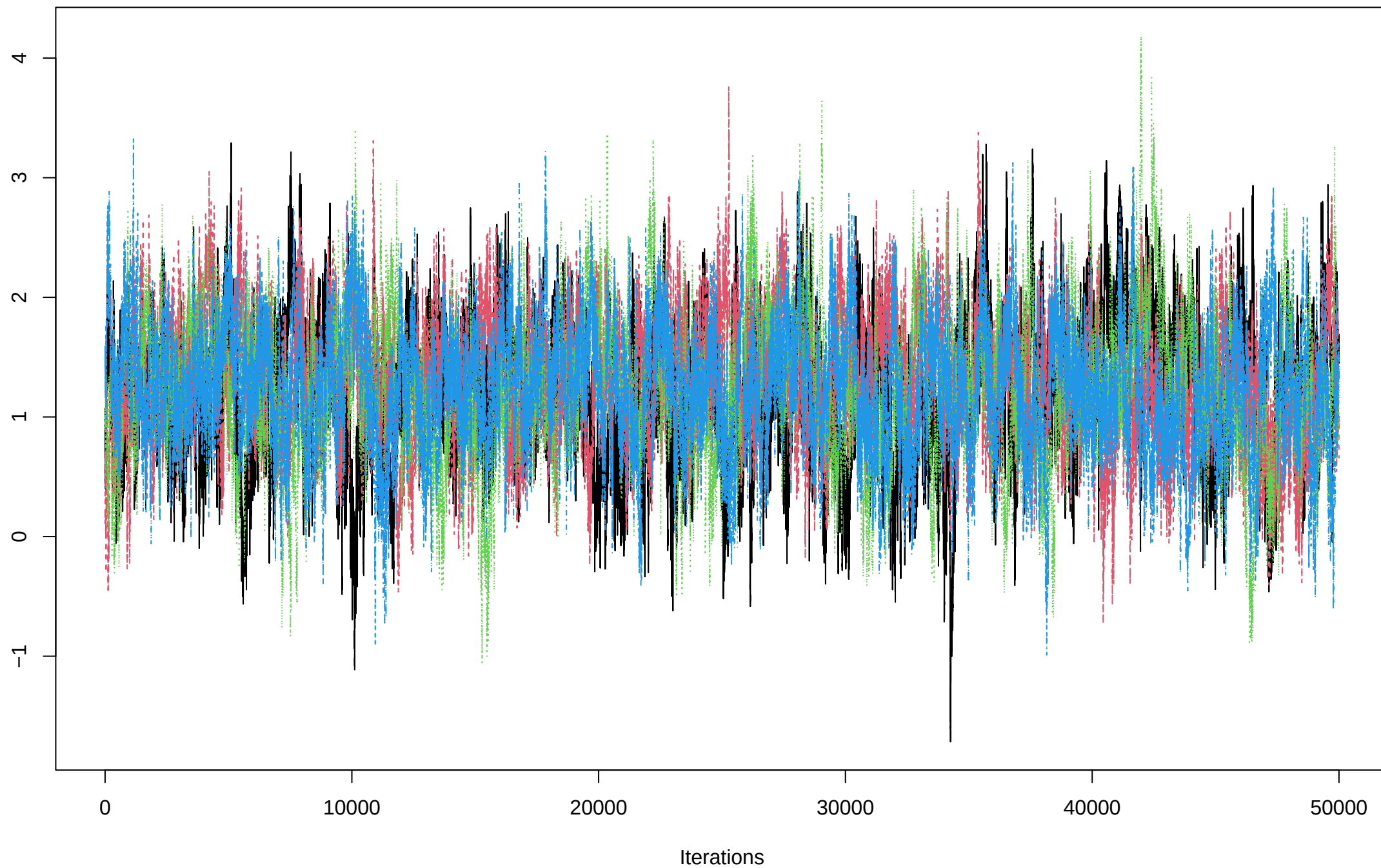
Trace of phi[8]
