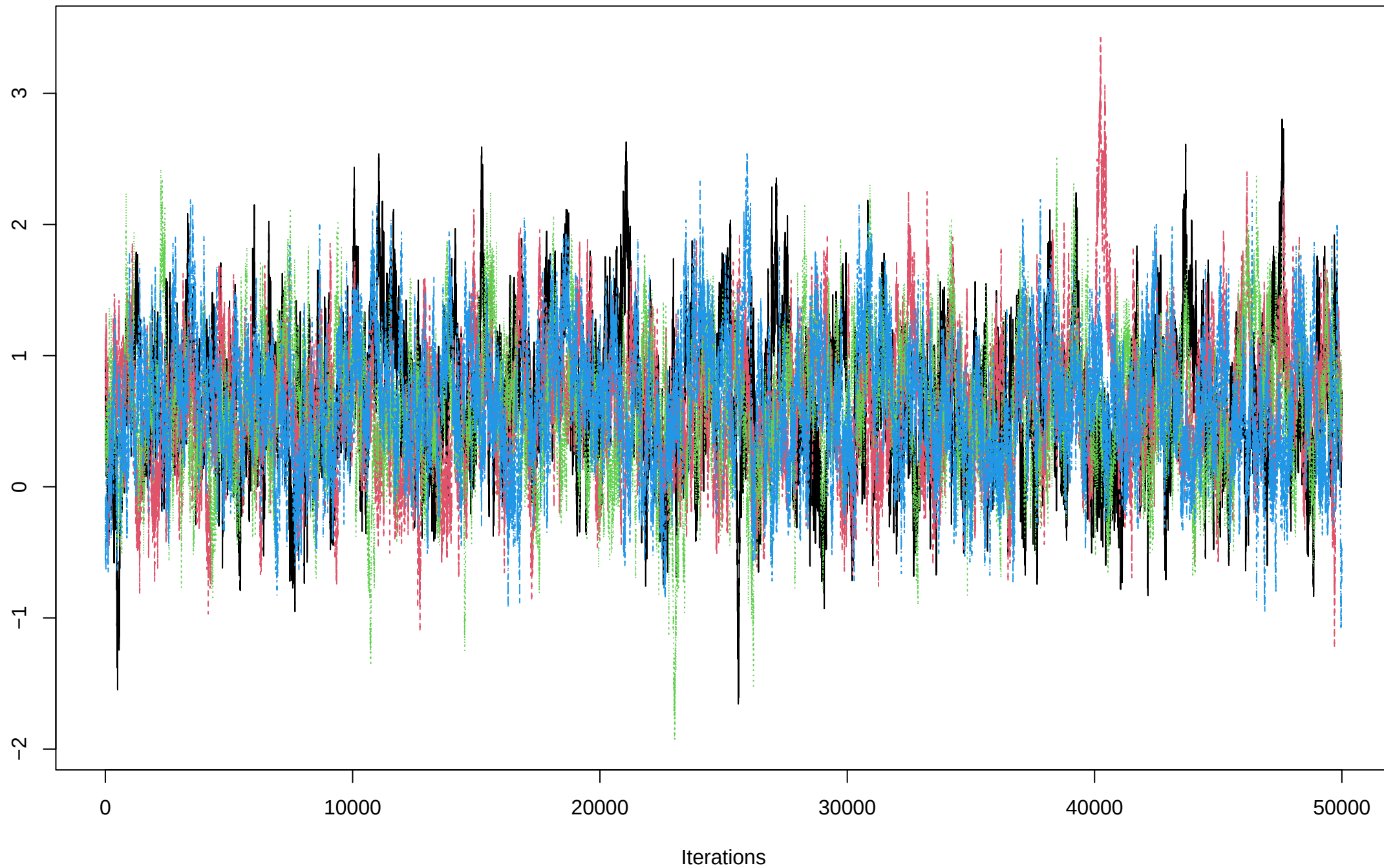
Trace of phi[4]
