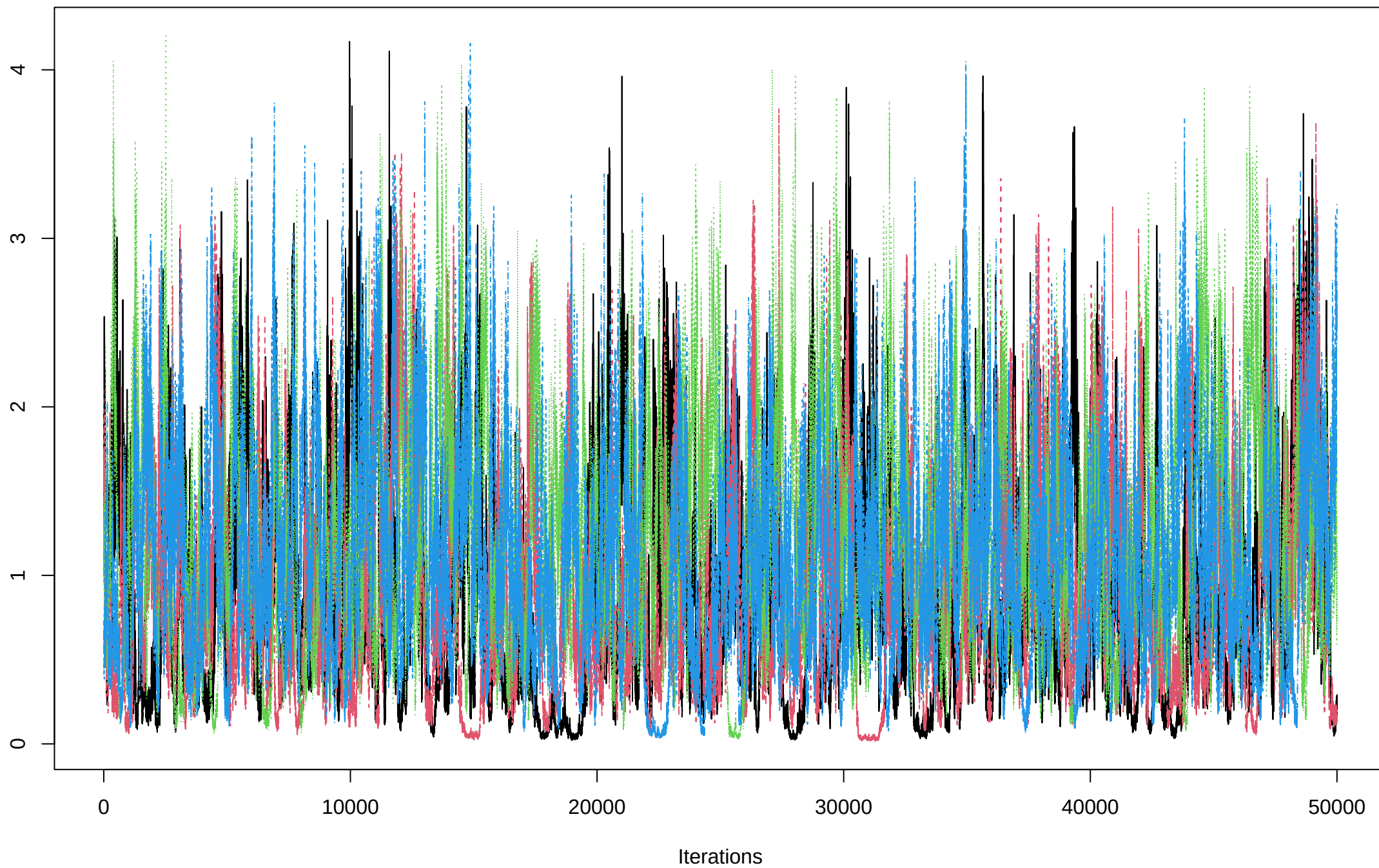
Trace of epsilon
