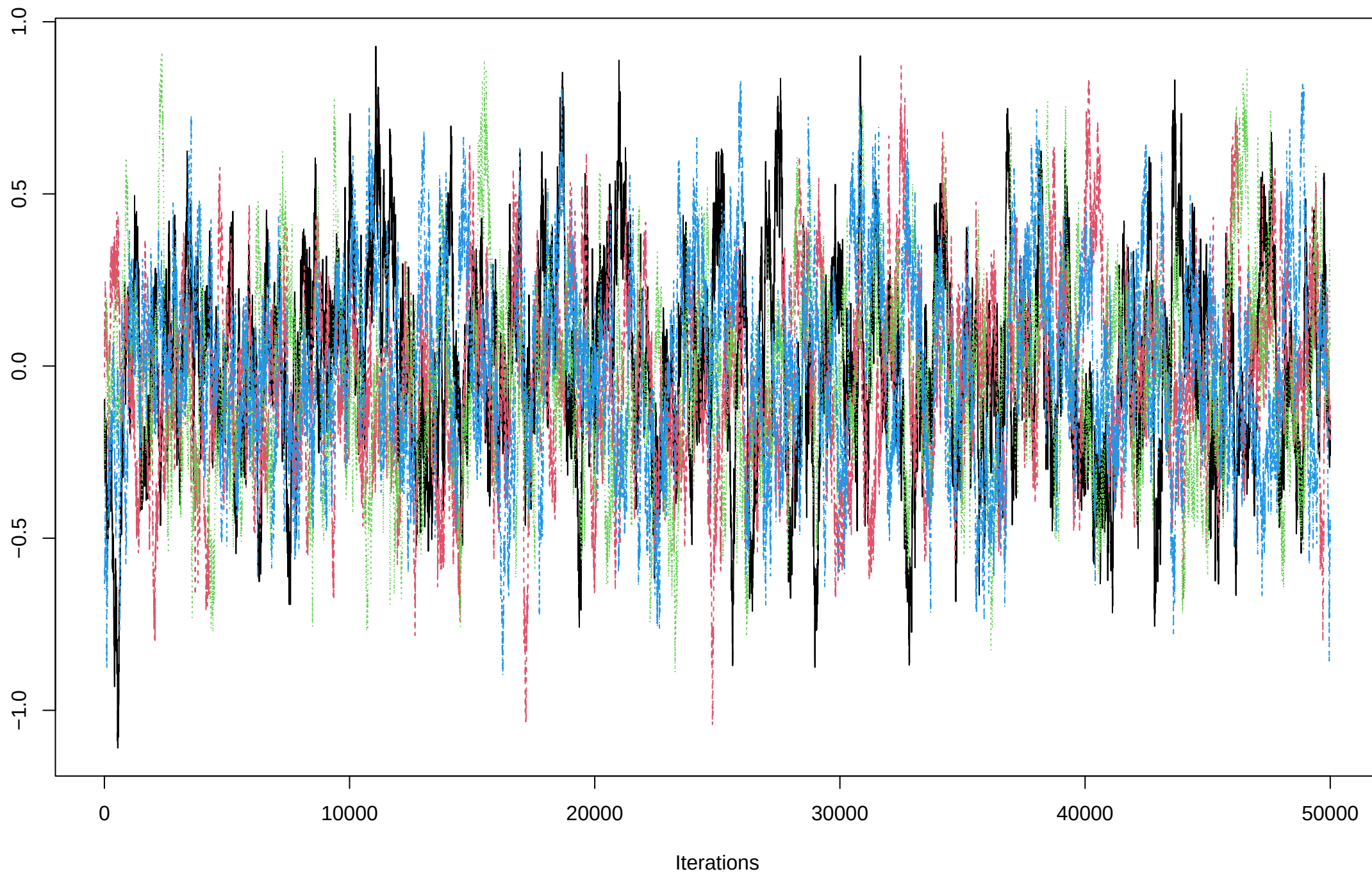
Trace of a[4]
