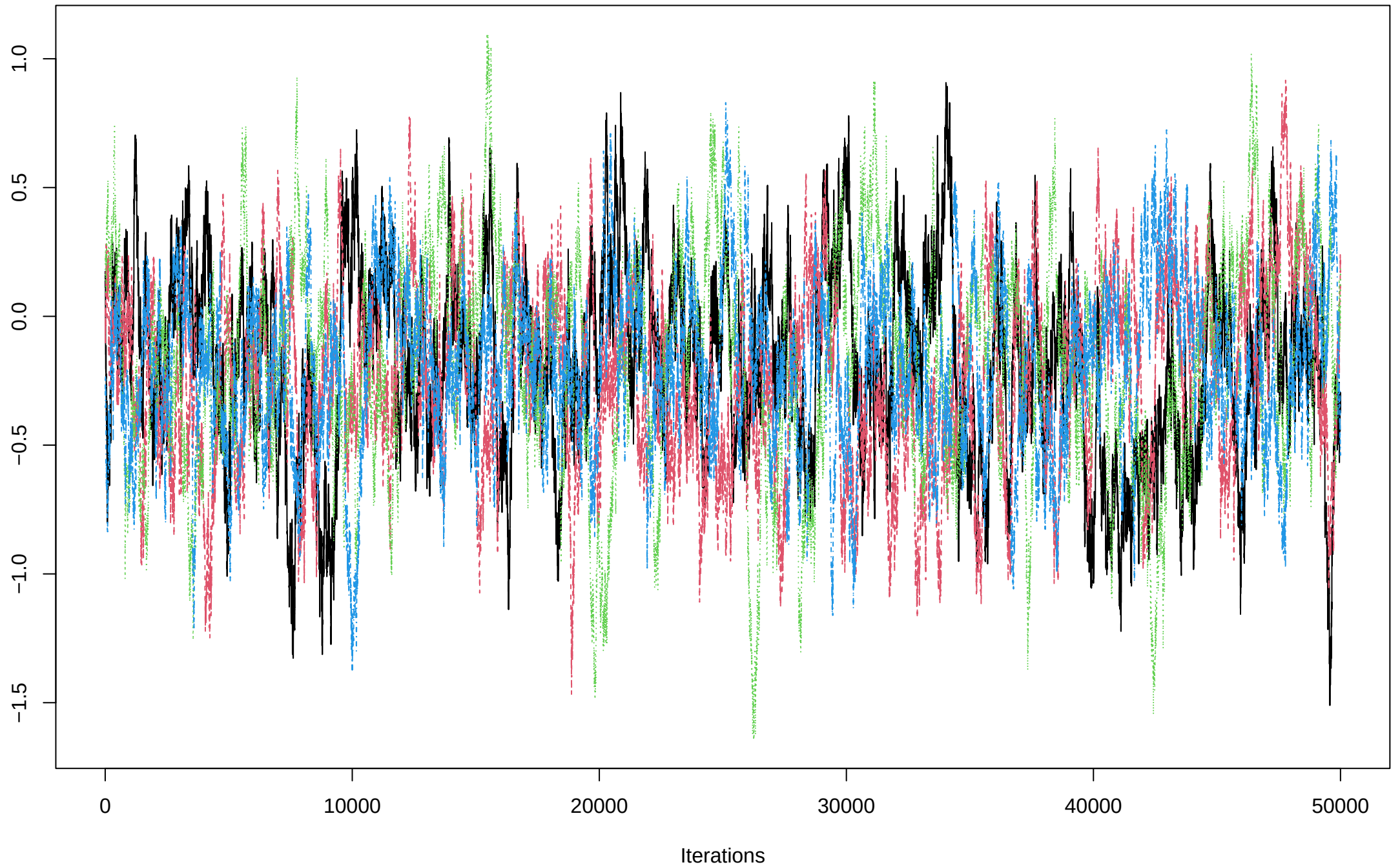
Trace of a[2]
