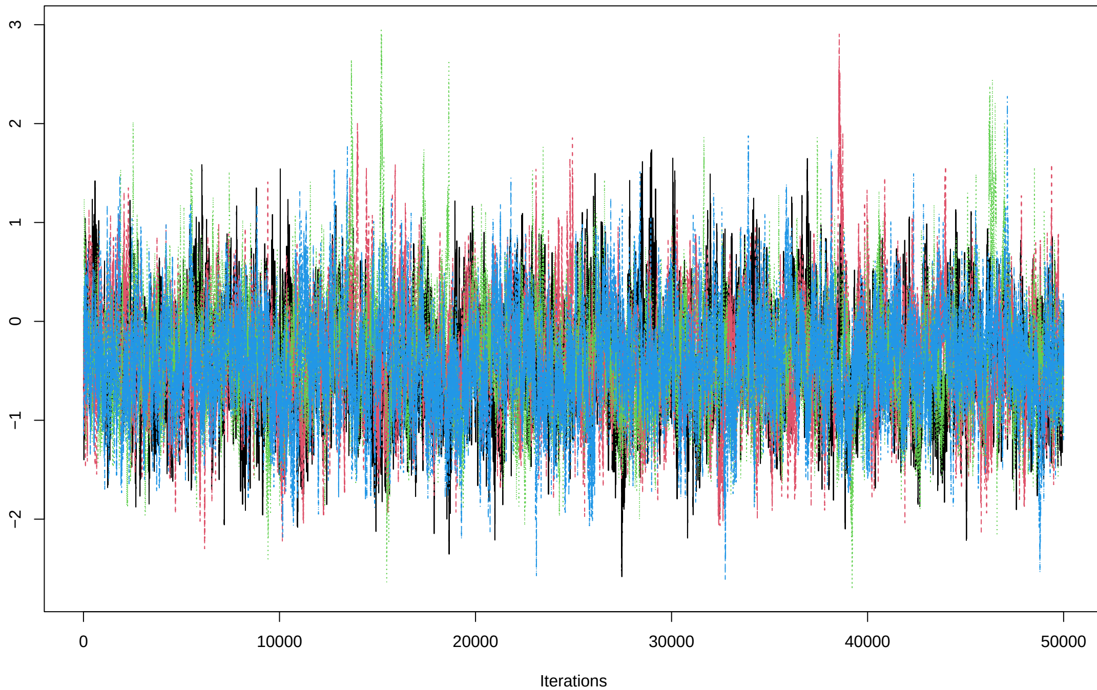
Trace of phi[23]
