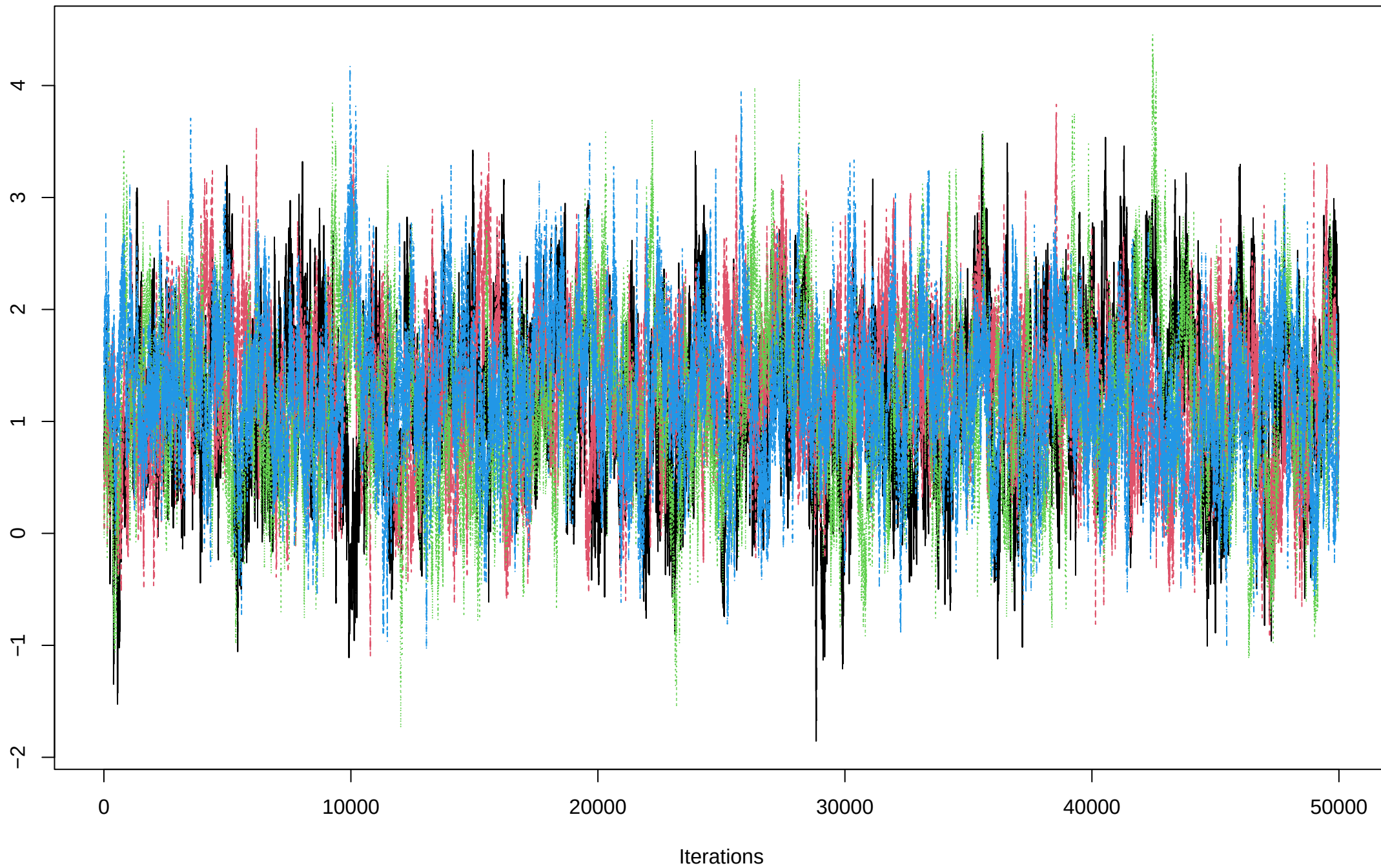
Trace of phi[12]
